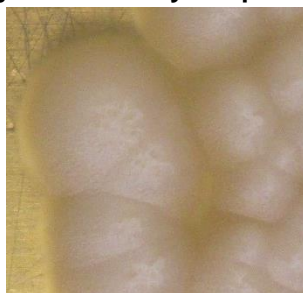
Figure 1: Colony Morphology
